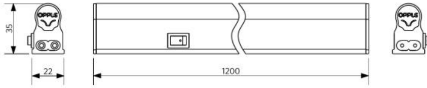
LED E T5 batten 1200
