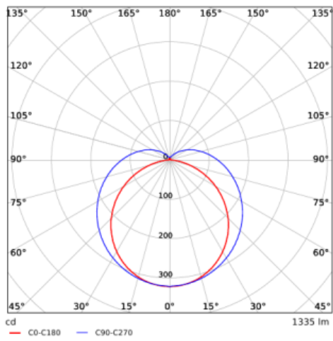
LED E T5 batten 1200
