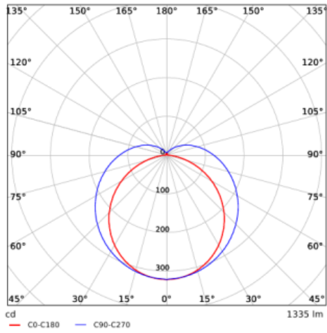
LED E T5 batten 1200
