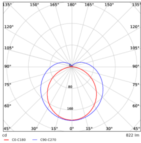
LED E T5 batten 600
