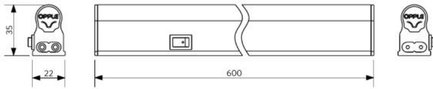
LED E T5 batten 600
